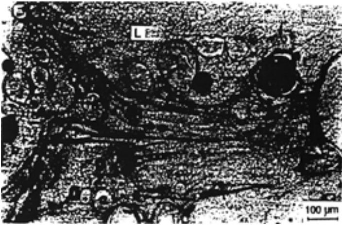
Figure 6: Lechatelierite matrix (L) with flow structures and enclosed air bubbles. (All photographs are taken from thin sections: normal transmission light.)
