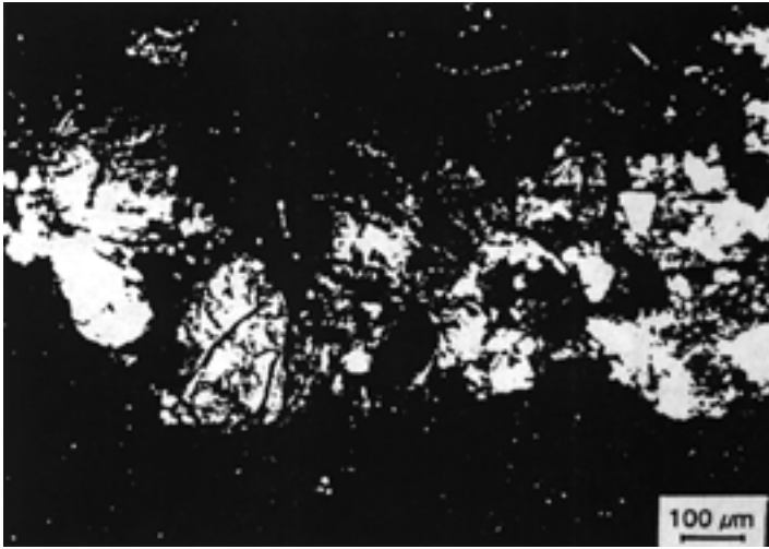
Figure 10: Thin section of the external part of a fulgurite. The glassy lechatelierite matrix is seen in the upper part of the photograph. In the middle, there are quartz grains that are partially transformed into lechatelierite or into cristobalite. The lower part of the photograph shows the sample porter (polarized light).
