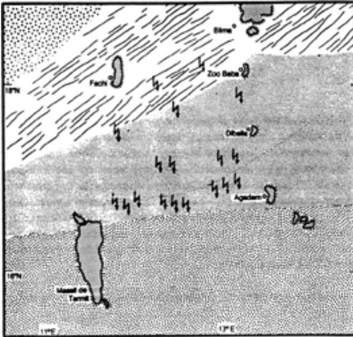
Figure 1: The study area in eastern Niger. Fulgurites are most common in the fossil dune complexes of the southern Sahara. The distribution pattern of lightning symbols shows the decrease in fulgurite concentration to the north. Definite results on fulgurite concentration in the vegetation-covered fossil dunes farther to the south are not yet available.
