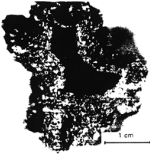
Figure 4: Cross section of a fulgurite. The lechatelierite matrix and the cortex of melted and partially transformed quartz grains surround the central tubular void. The four-point shape was formed during the collapse of the central void, caused by the surrounding pressure immediately after the lightning passage and substrate melting.
