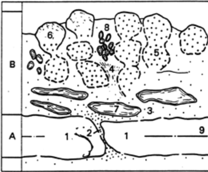
Figure 5: Longitudinal section of a fulgurite (schematic): (1) central tubular void, parallel to the longitudinal axis of the fulgurite (9), diameter 1-2 cm (A); (2) glass bridge (lechatelierite); (3) lechatelierite matrix (Figure 6); (4) flow structures (Figure 6); (5) former quartz grains, melted with preserved contours (Figure 7); (6) quartz grains, partially transformed into cristobalite (Figure 10); (7) large flattened air bubbles near the central void (Figure 8); (8) small air bubbles (Figure 9); (9) longitudinal axis of the fulgurite; (A) diameter of the central tubular void: 1-2 cm; (B) thickness of the fulgurite crust: 3-4 mm maximum.
